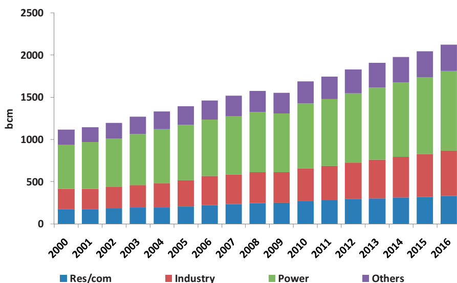
Non-OECD Sectoral Gas Demand 2000-16
