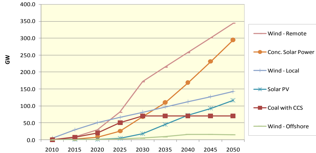
New Technology Capacity - Lieberman-Warner: Case A
