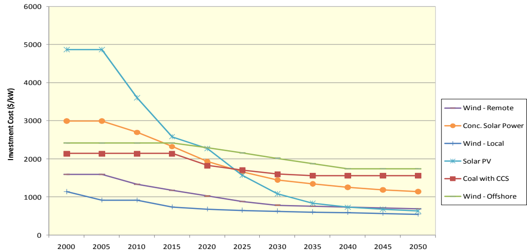
Technology Learning Results - Lieberman-Warner: Case A
