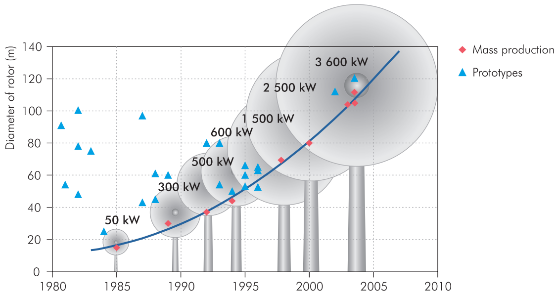
Figure 4.11 ▶ Development of wind turbine size
