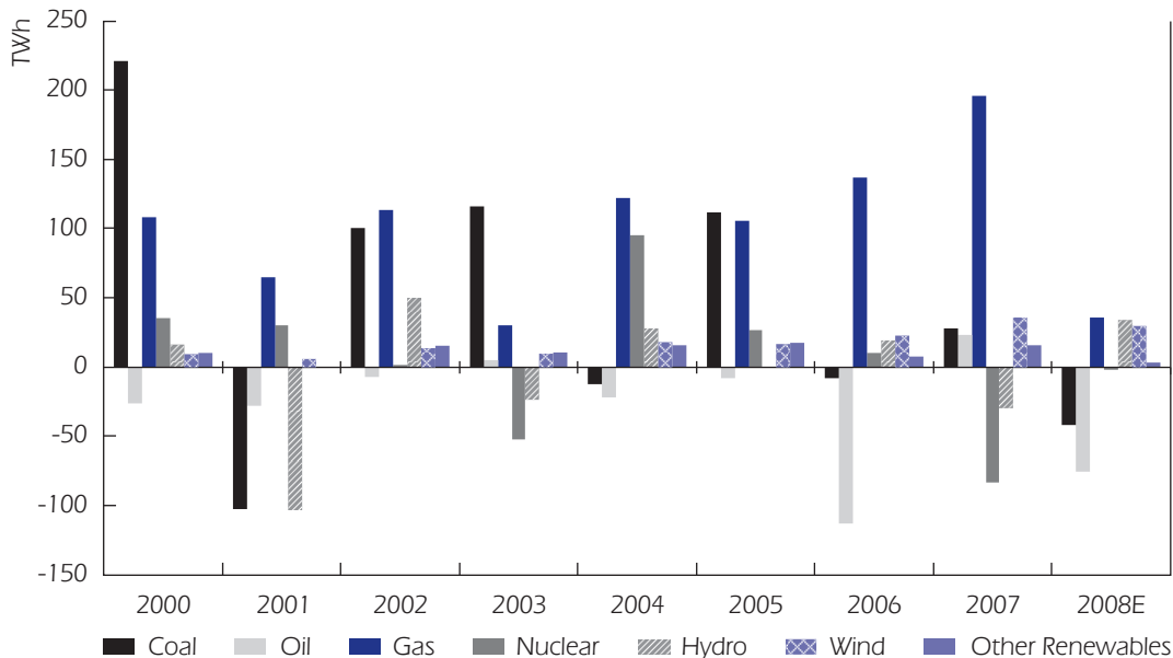
Figure 16 Changes in power generation by fuel source in OECD
