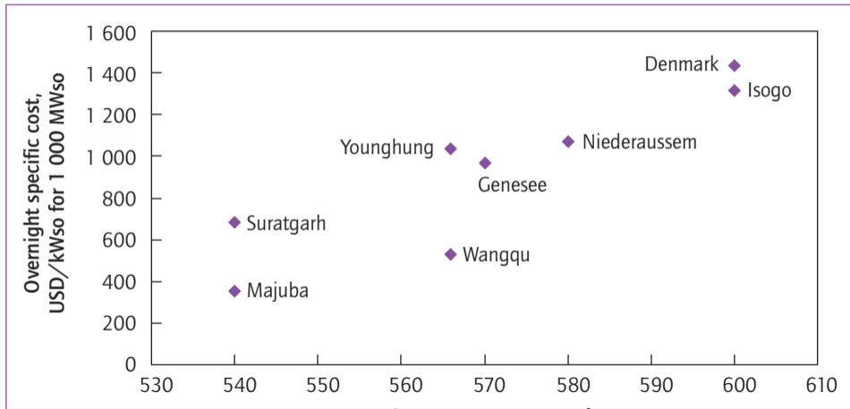
Figure 29 • Adjusted specific plant costs versus main steam temperature
